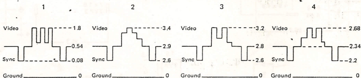
TYPICAL INPUT WAVEFORM
